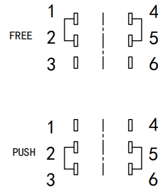
CIRCUIT DIAGRAM
