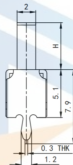
SCHEMATIC (SHORTING)
