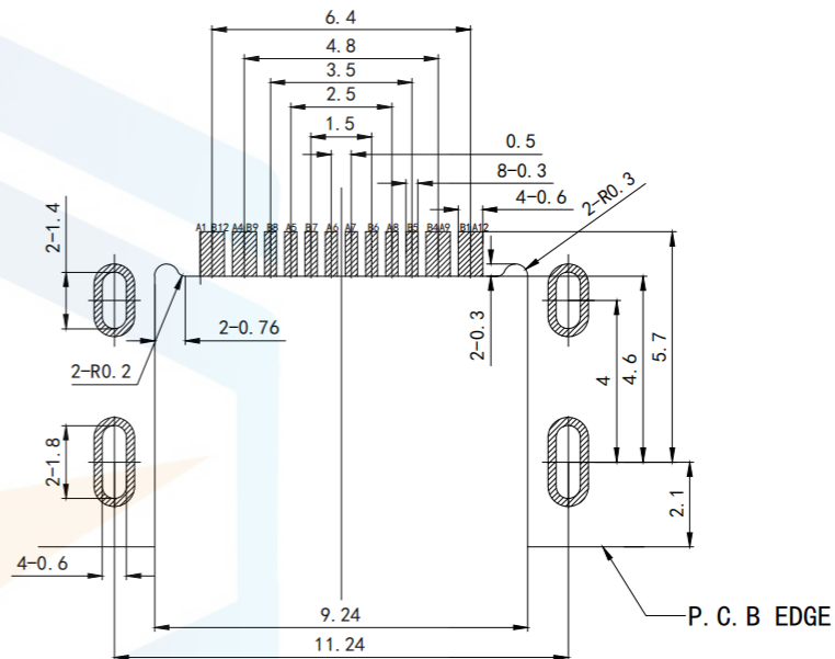
RECOMMENDED PCB LAYOUT (COMPONENT SIDE) TOLERANCE UNSPECIFIED \pm 0.05\text{mm}
