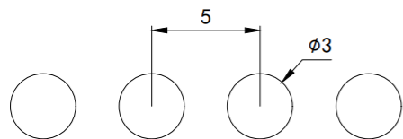
RECOMMENDED P. C. B LAYOUT ( \pm 0.05 )
