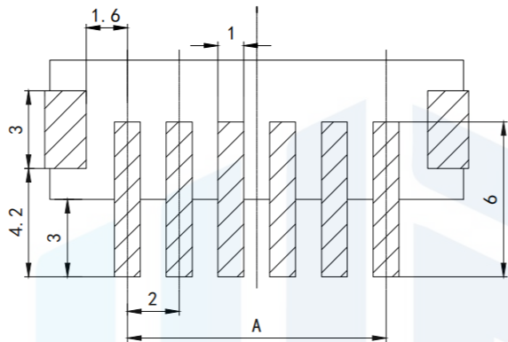
RECOMMENDED P. C. BOARD LAYOUT (TOP VIEW) GENERAL TOLERANCE: \pm 0.05
