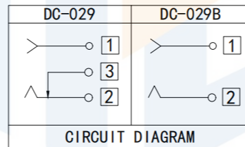
Circuit Diagram □:Terminal No.
