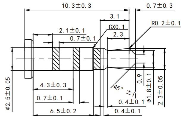
φ2.5mm 4 POLE PLUG DETAIL DRAWING
