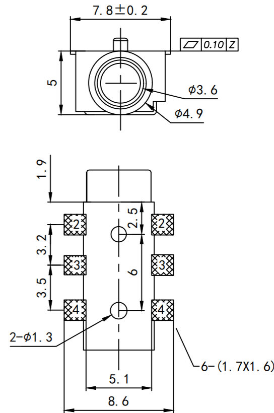
P. C. B LAYOUT TOP VIEW
