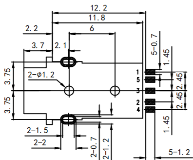
RECOMMEND PCB LAYOUT TOP VIEW
